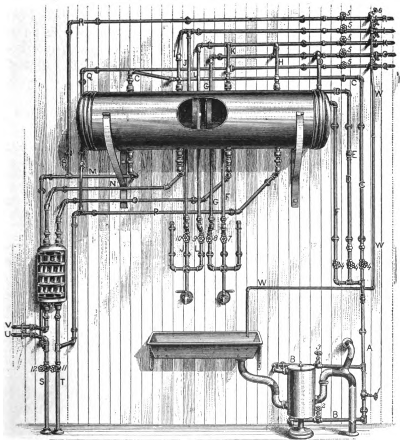
Horizontal Double Boiler.
