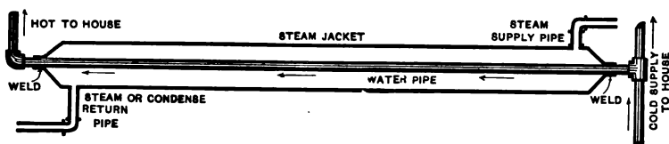
Boiler Heated by Steam.
