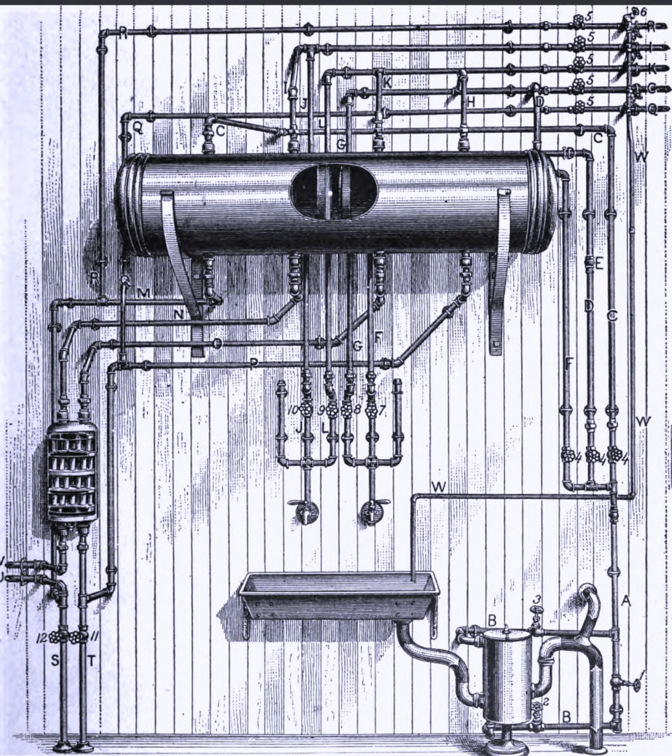
Kitchen boiler connections
