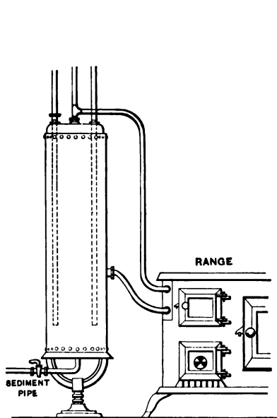
Fig. 1.—Side and Top Connections.
