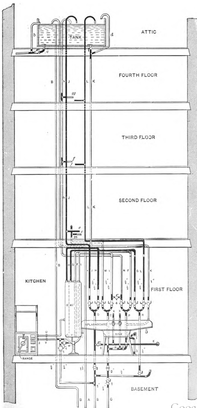
Double Boiler System of Plumbing.
