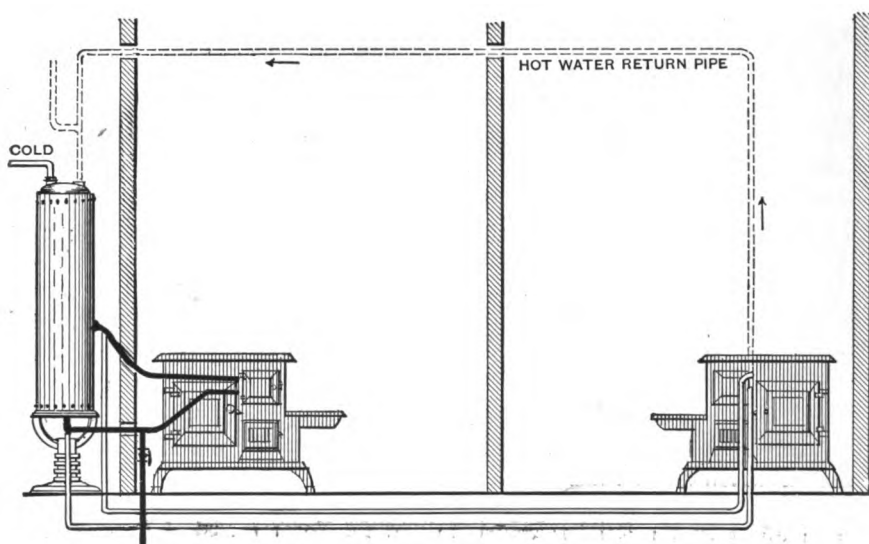
Piping from Stove to Boiler in Different Room.
