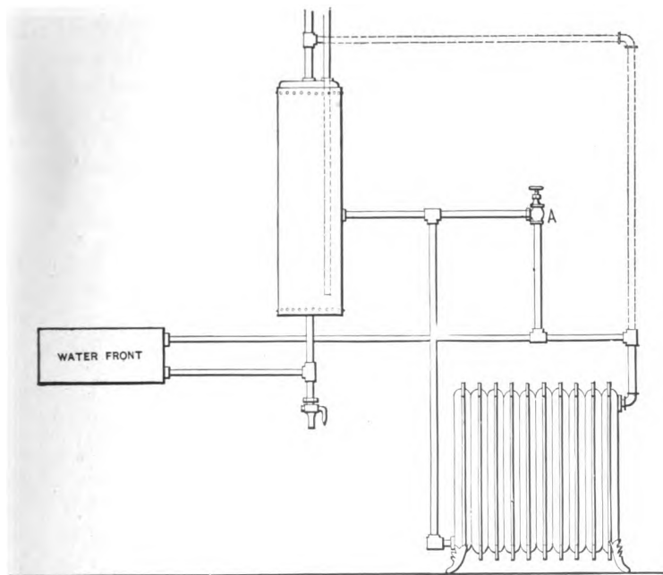
Radiator Below Water Front.
