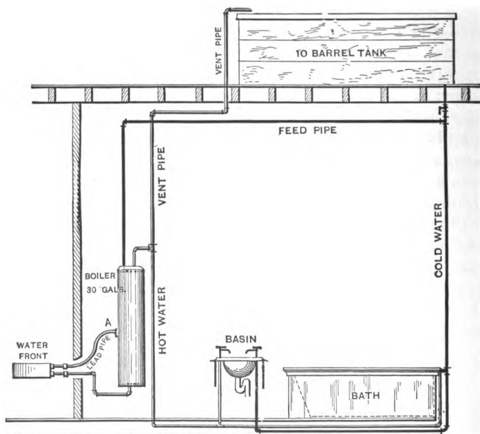
A Noisy Range Boiler.
